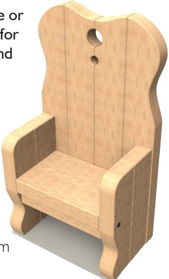
Story Telling Chair L 780 W 485 H 1400mm
